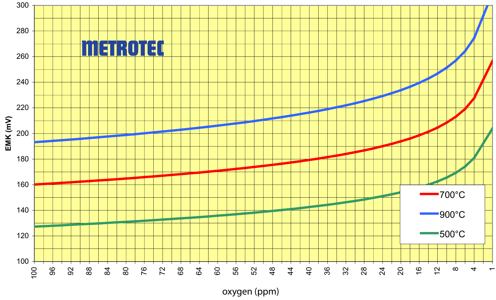
EMF of oxygen sensors vs. concentration at different temperatures
