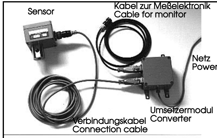
Connections to the A15 sensor
